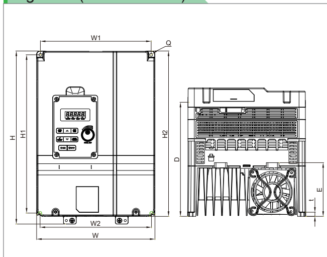
Figure C (IP20 Frame 3)
