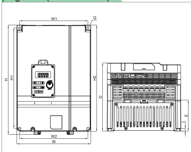
Figure D (IP20 Frame 4)
