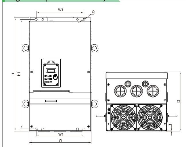
Figure F (IP20 Frame 6)
